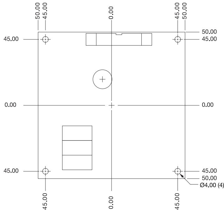
Control PC Board Dimensions (mm)
