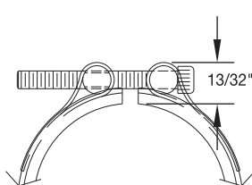
< 2" ID — 6-32 Screw
