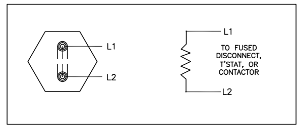
TYPICAL WIRING 1 ELEMENT – SINGLE PHASE
