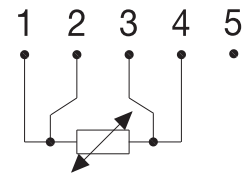
RTD- PT100, PT1000 4-wire
