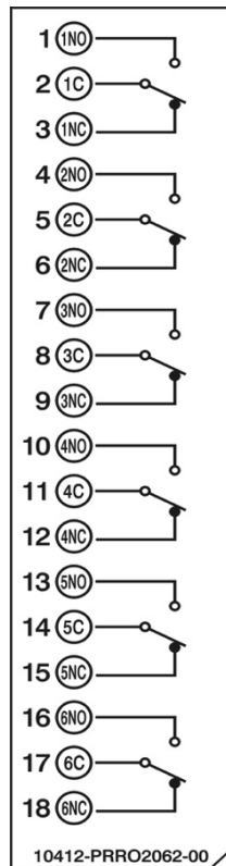
Relay output card PPS90003/RO206
