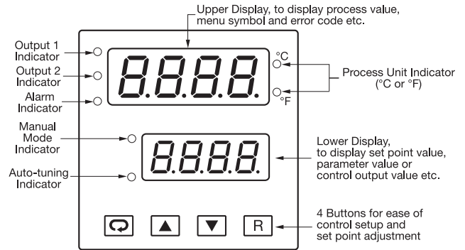
Figure 1.3 Front Panel Description
