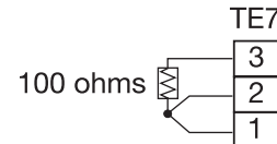
Figure 5–1 RTD Calibration
