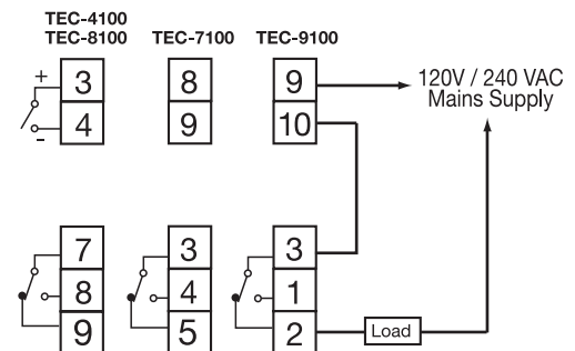
Dwell Timer Function Wiring Diagram
