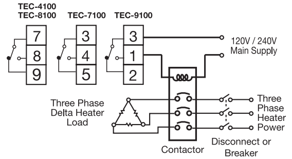
Figure 2.20 Alarm Output to Drive Contactor
