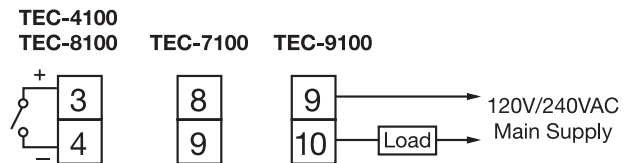
Figure 2.9 Output 1 Relay (2A, 240V Max.) or Triac (1A, 240V Max.) (SSR) to Drive Load
