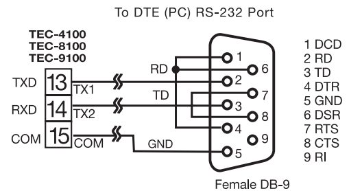
Figure 2.23 Configuration of RS-232 Cable
