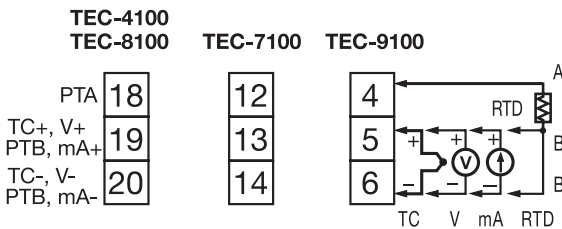
Figure 2.8 Sensor Input Wiring
