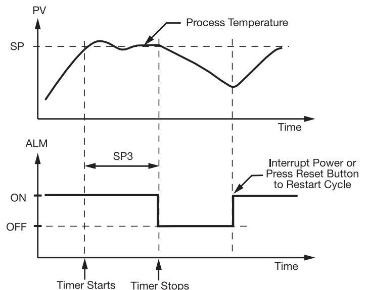
Figure 3.6 Dwell Timer Function
