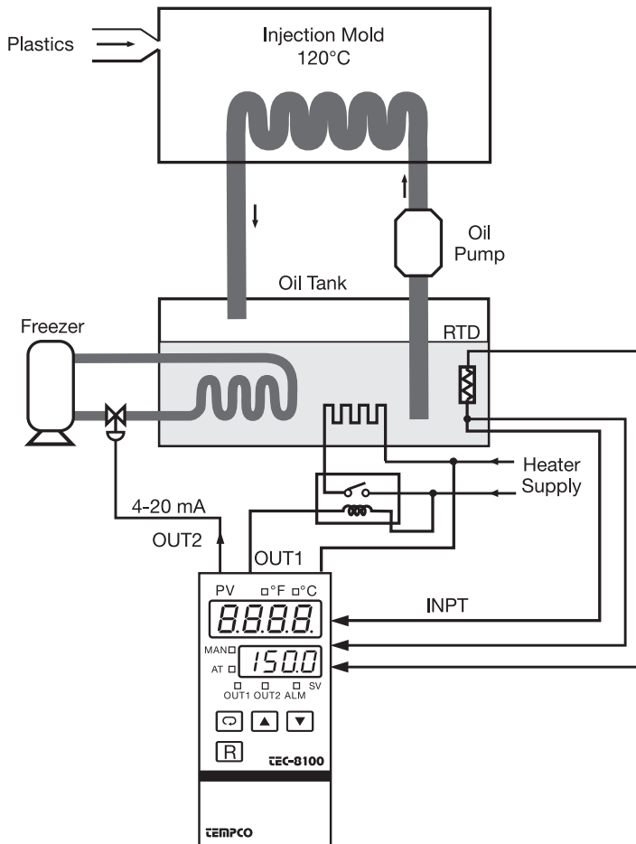
Figure 4.3 Heat-Cool Control Example
