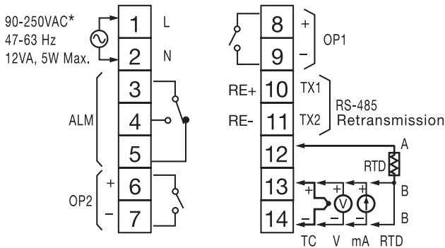
Figure 2.5 Rear Terminal Connection for TEC-7100
