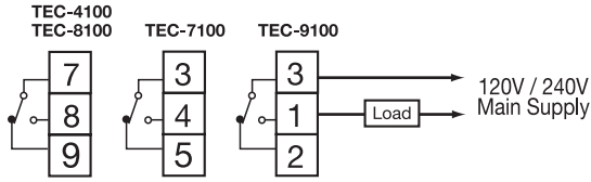
Figure 2.19 Alarm Output to Drive Load
