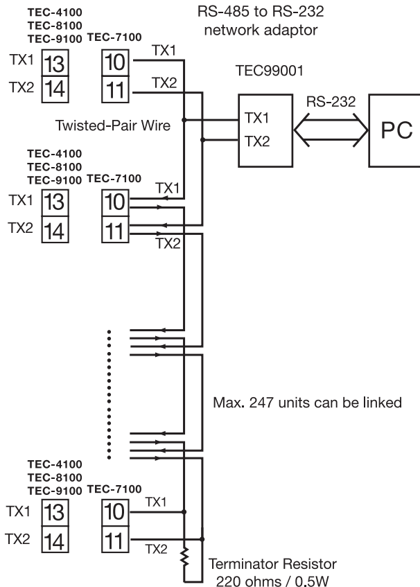
Figure 2.21 RS-485 Wiring
