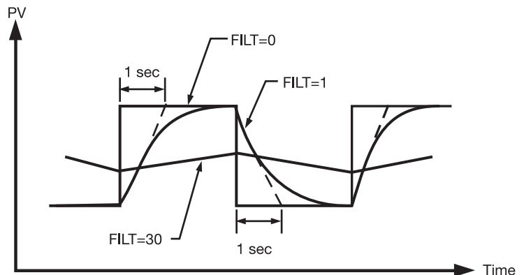
Figure 3.8 Filter Characteristics
