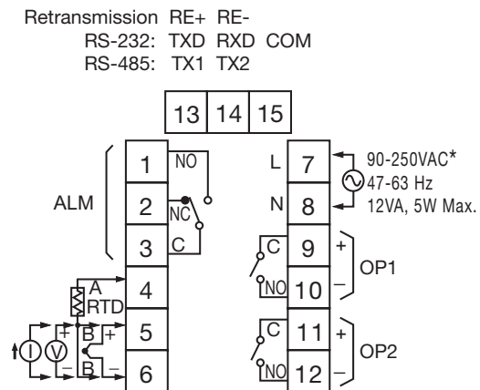
Figure 2.6 Rear Terminal Connection for TEC-9100
