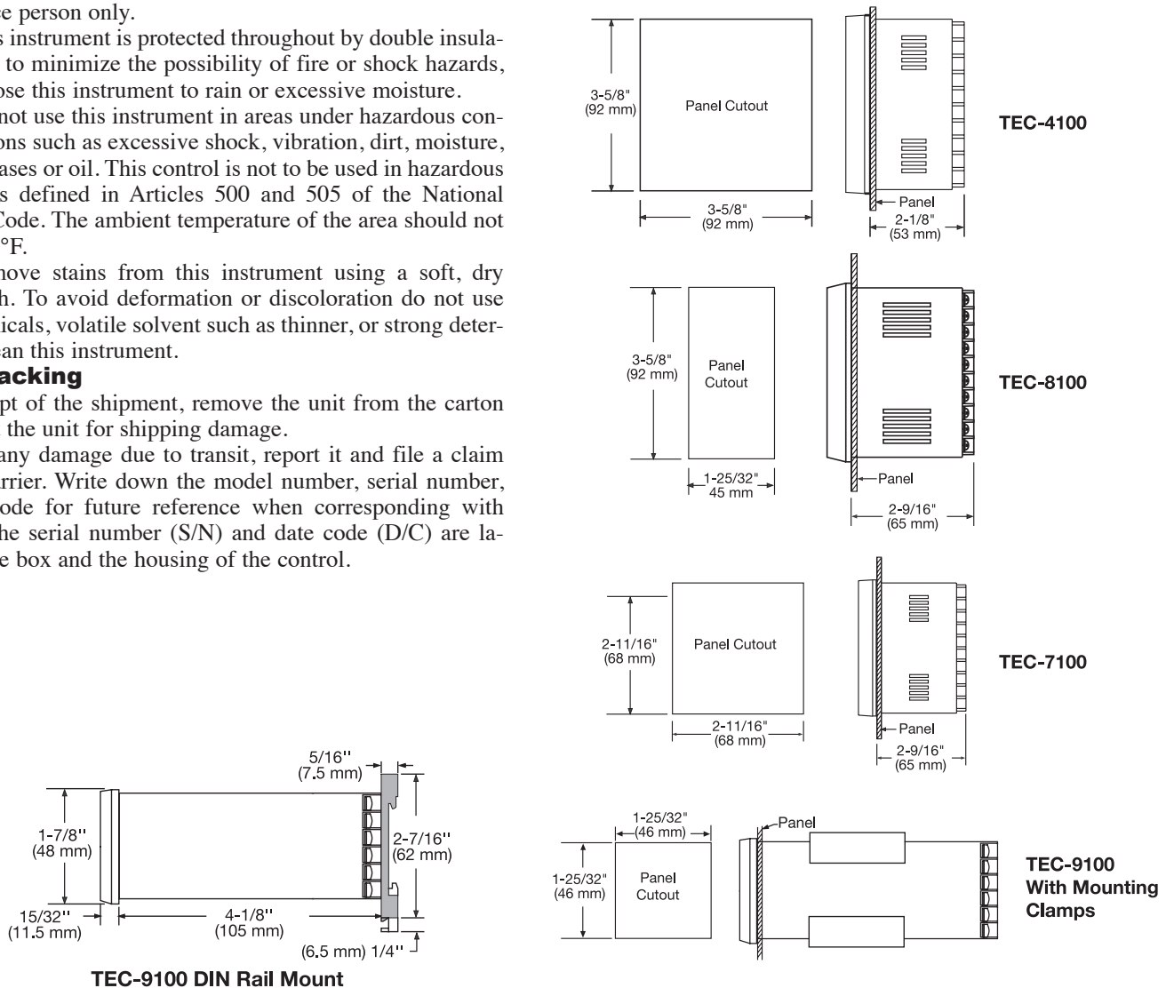
Figure 2.1 Mounting Dimensions
