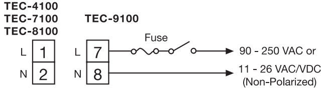
Figure 2.7 Power Supply Connections
