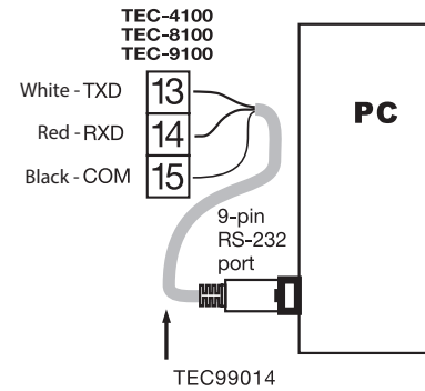
Figure 2.22 RS-232 Wiring
