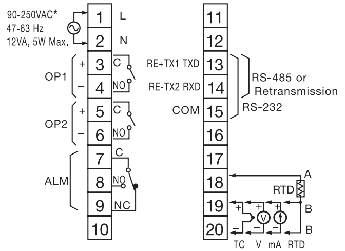
Figure 2.4 Rear Terminal Connection for TEC-4100 and TEC-8100
