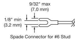
Figure 2.2 Lead Termination for TEC-4100, TEC-8100 and TEC-7100
