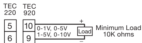
Figure 2.12 Output 1 Linear Voltage
