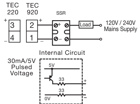
Figure 2.15 Output 2 Pulsed Voltage to Drive SSR
