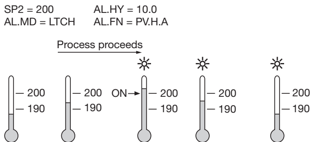
Figure 3.4 Latching Process Alarm
