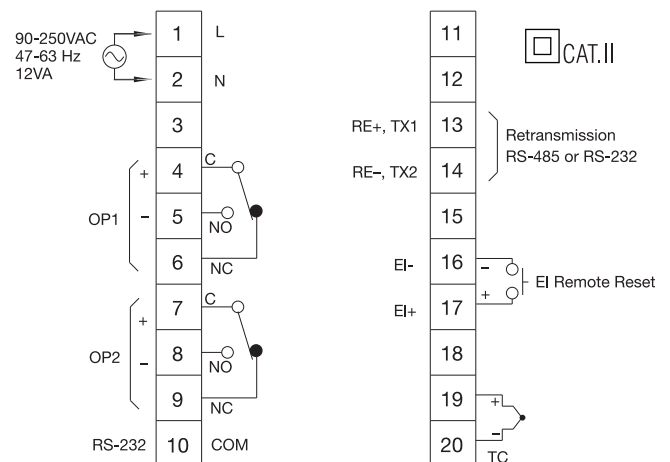
Figure 2.2 Lead Termination
