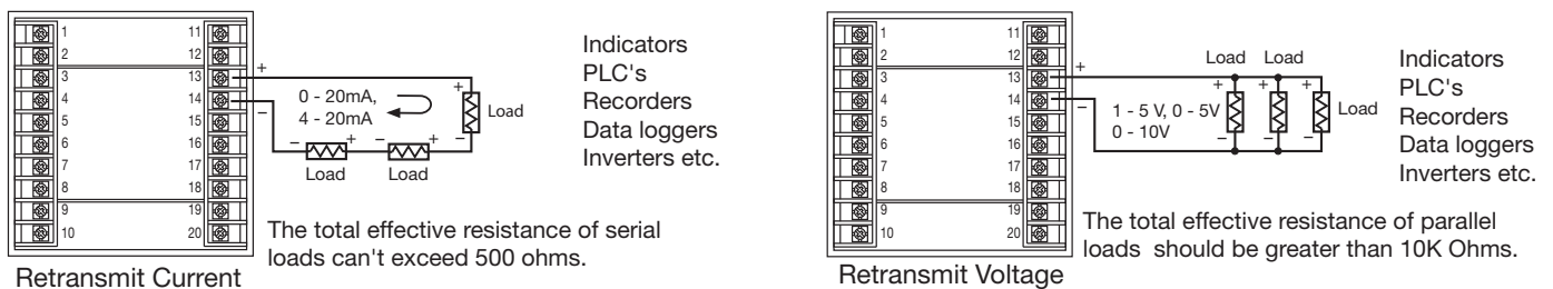
Figure 2.15 Retransmission Wiring
