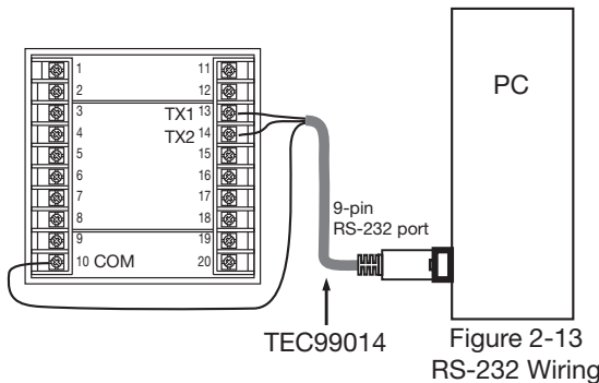
Figure 2.13 RS-232 Wiring
