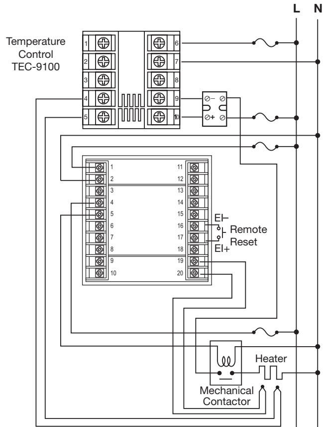
Figure 4.1 Over-Temperature Protection with Remote Reset
