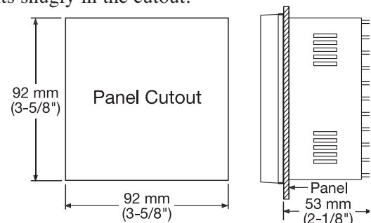
Figure 2.1 Mounting Diagram
